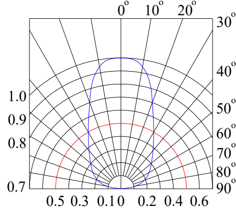
Radiation Diagram
